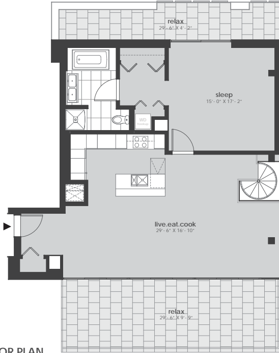
SIXTH FLOOR PLAN
